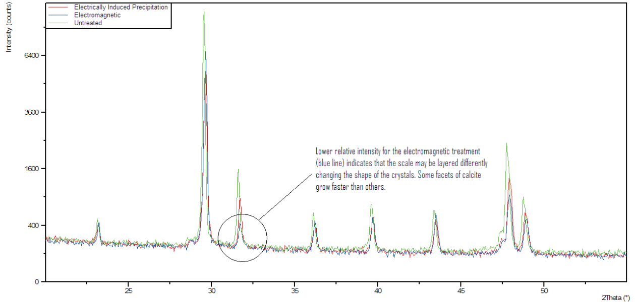
FIGURE 18: X-RAY DIFFRACTION RESULTS
