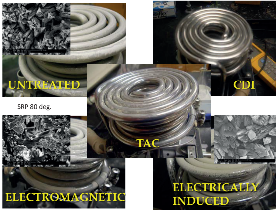
FIGURE 19: TEMPE TAP WATER (80 °C) SCALE ON ELEMENTS AND THROUGH SEM
