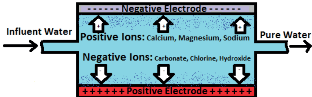
FIGURE 9: CDI REGENERATION
